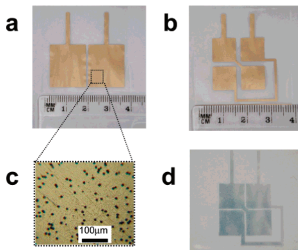
Figure 2. (a) Two gold pixels ( 1.5 \times 2 cm) patterned on a polycarbonate (PC) membrane. (b) A 2 \times 2 gold pattern ( 2 \times 2 cm) on PC. (c) Magnification ( 80\times ) of the metallized membrane to show the unfilled pores. (d) Image of the pattern on the glass backing plate used during the evaporation process indicating that the gold passes through the membrane during deposition.
