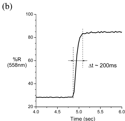
Figure 6. (a) Temporal change in %R (1540 nm) during electrochromic switching of a D3 type reflective device between -1 and +1 V every 5 (upper) and 1 (lower) seconds. (b) A single transition illustrating the switching time of the same device ( -1 to +1 V, \lambda = 558 nm).
