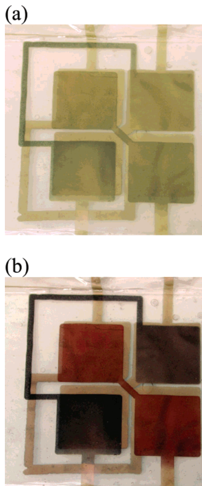
Figure 9. A 2 \times 2 pixels patterned device (D6 type) comprising two cathodically coloring electrochromic polymers to provide color match/contrast. (a) Both polymers oxidized (bleached), and (b) both polymers reduced (colored).
